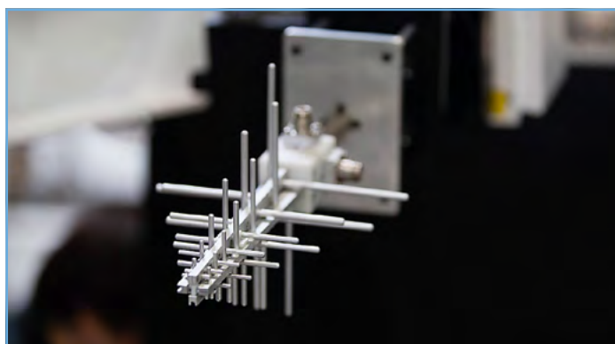
Antennenintegration
