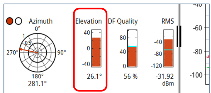
Fig. 6. Display of elevation during a measurement with the SignalShark and ADFA.
