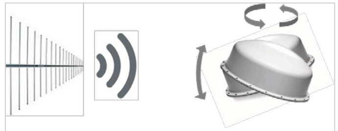
Fig. 9. Narda antennas are both rotated and tilted during the determination of the phase catalog.
