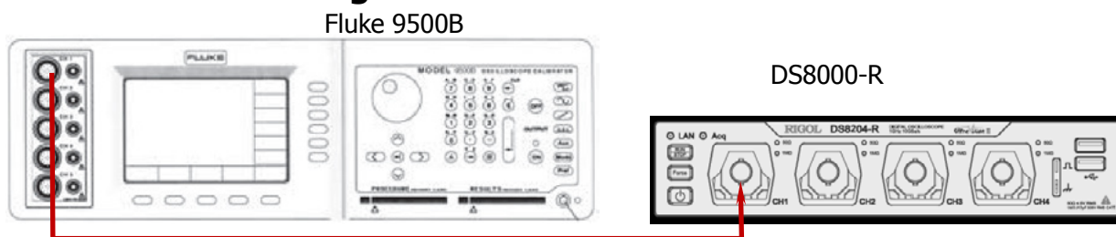
Figure 2-4 Bandwidth Limit Test Connection Diagram
