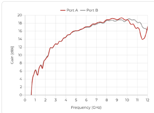
Gain
