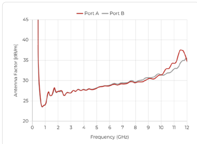
Antenna Factor
