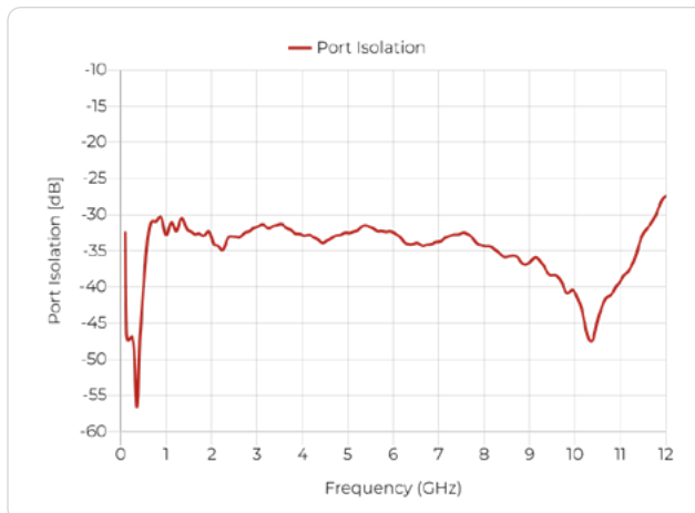
Port Isolation
