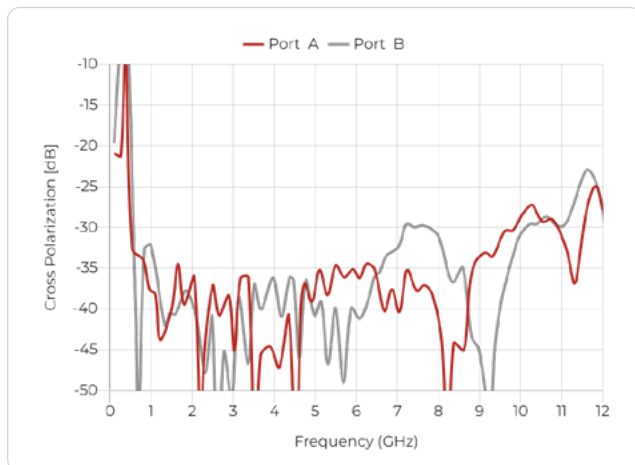
Cross Polarization
