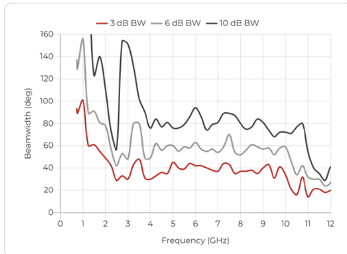
Port A, E plane
