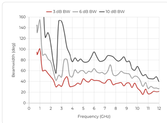
Port B, E plane
