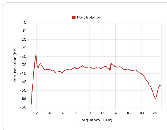
Port Isolation
