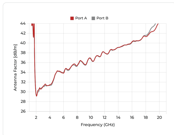
Antenna Factor
