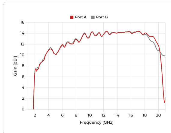
Gain
