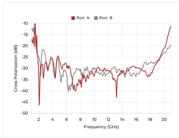
Cross Polarization
