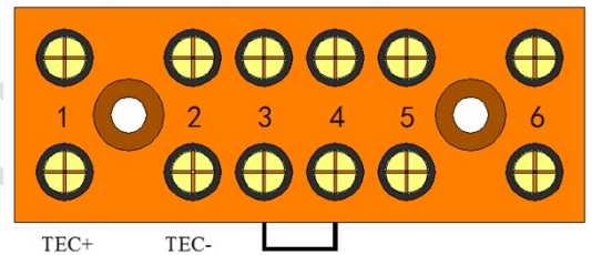
Wiring Schematic (Power Connector)
