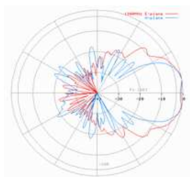
1900 MHz
