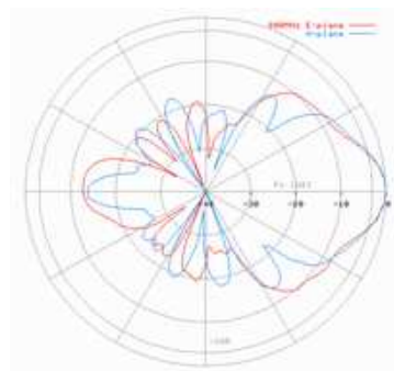
800 MHz
