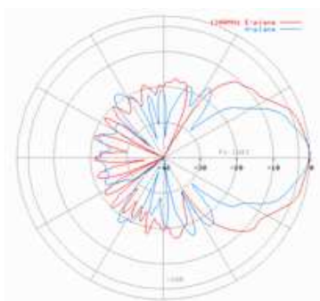
1300 MHz
