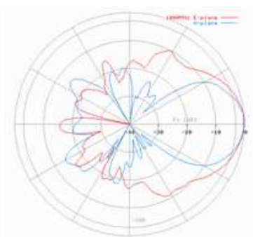
1000 MHz
