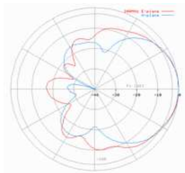
300 MHz
