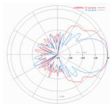
1600 MHz
