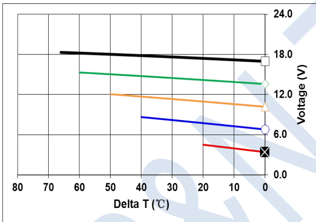
Performance Curves Th=25 °C (性能曲线 Th=25°C)
