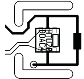
Example of HTU20D(F) sensor mounting with slits mills to minimize heat transfer
