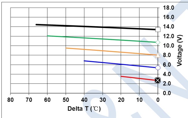
Performance Curves Th=25 °C (性能曲线 Th=25°C)
